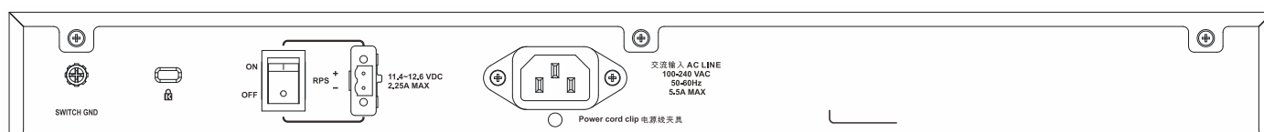
Figure 1-26 Rear panel view of a DGS-3000-28XMP Switch
