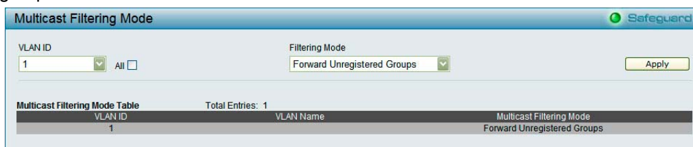
Figure 75 – Configuration > Multicast Filtering Mode
