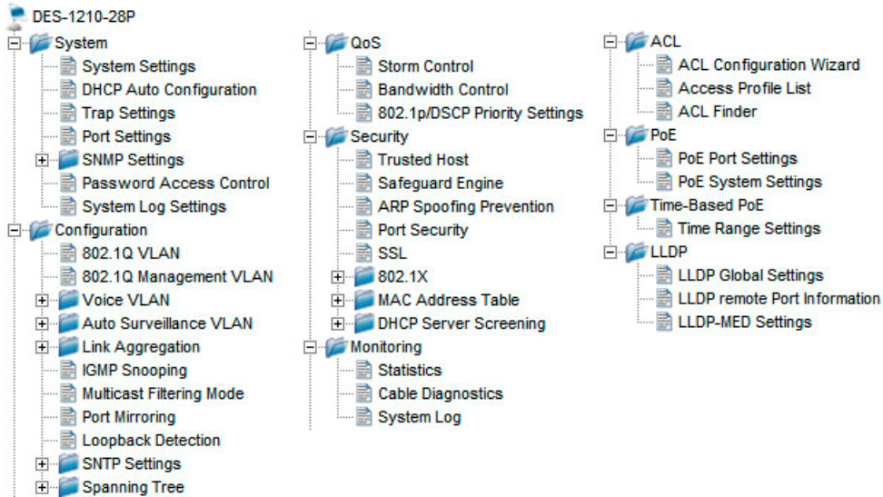
Figure 43 –Function Tree
