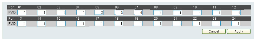
Figure 66 – Configuration > 802.1Q VLAN > Asymmetric VLAN – Assign PVID
