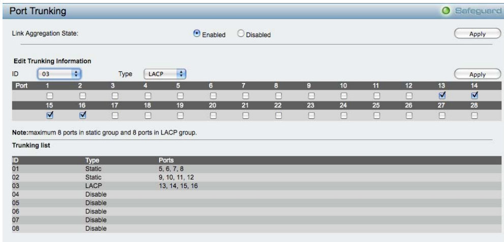
Figure 70 – Configuration > Link Aggregation > Port Trunking
