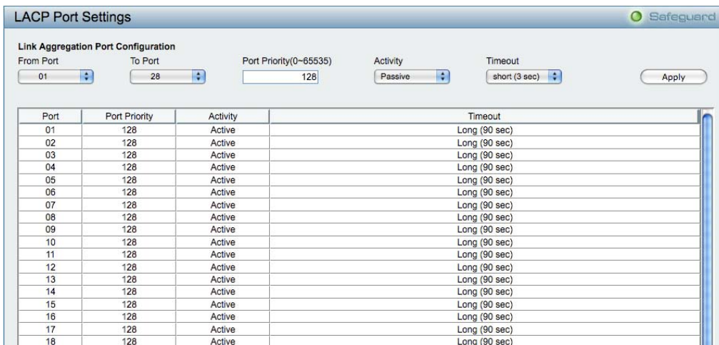
Figure 71 – Configuration > Link Aggregation > LACP Port Settings
